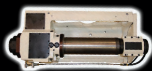
Regulating wheelhead
