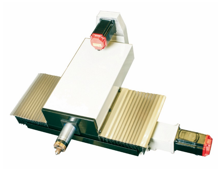
Two-Axis CNC Dresser
